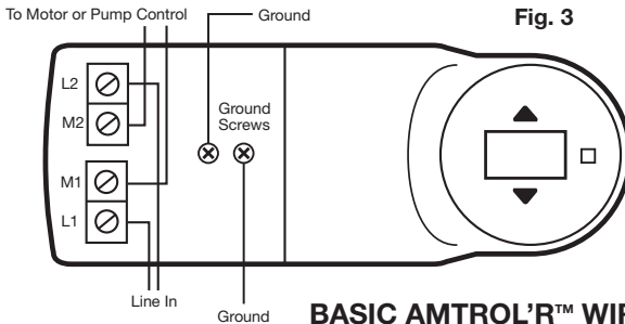
BASIC AMTROL'R™ WIRING
