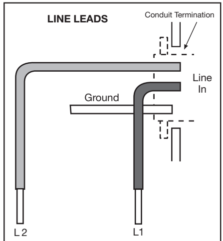
BASIC AMTROL'R™ WIRING
